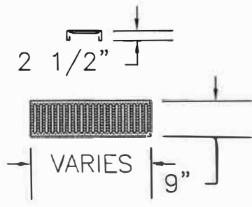
GRATING DETAIL NOTE: * VARIES WITH CHAMBER LENGTH
