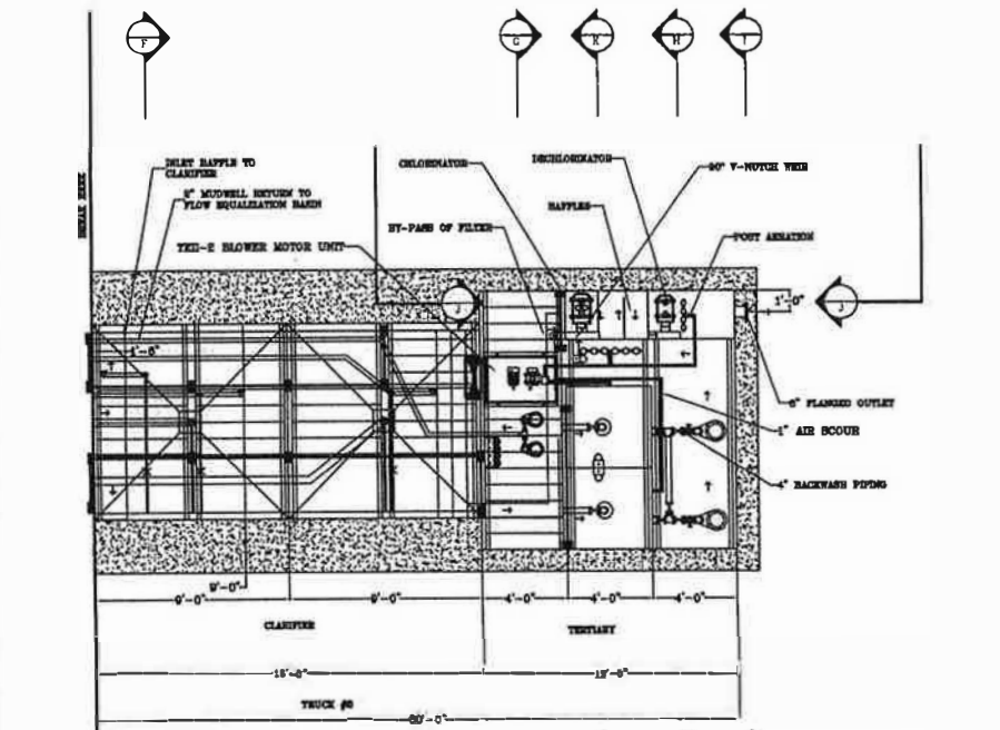
PLAN VIEW
