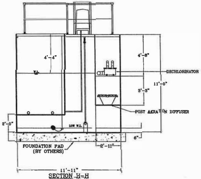
SECTION H-H FILTER/ DE-CHLORINATOR
