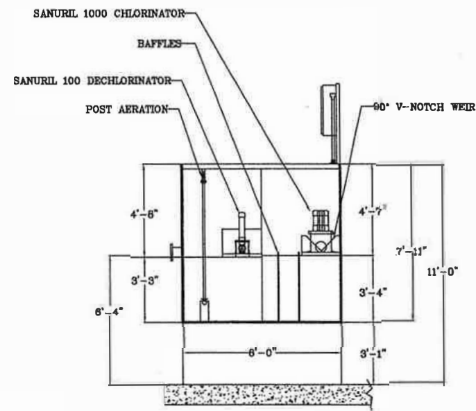
SECTION -J-J CL2 TANK
