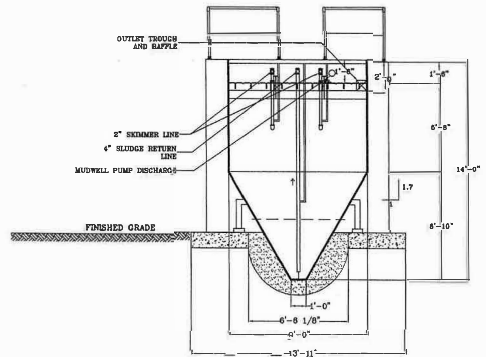
SECTION F-F CLARIFIER OUTLET END
