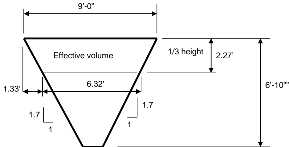
END VIEW
