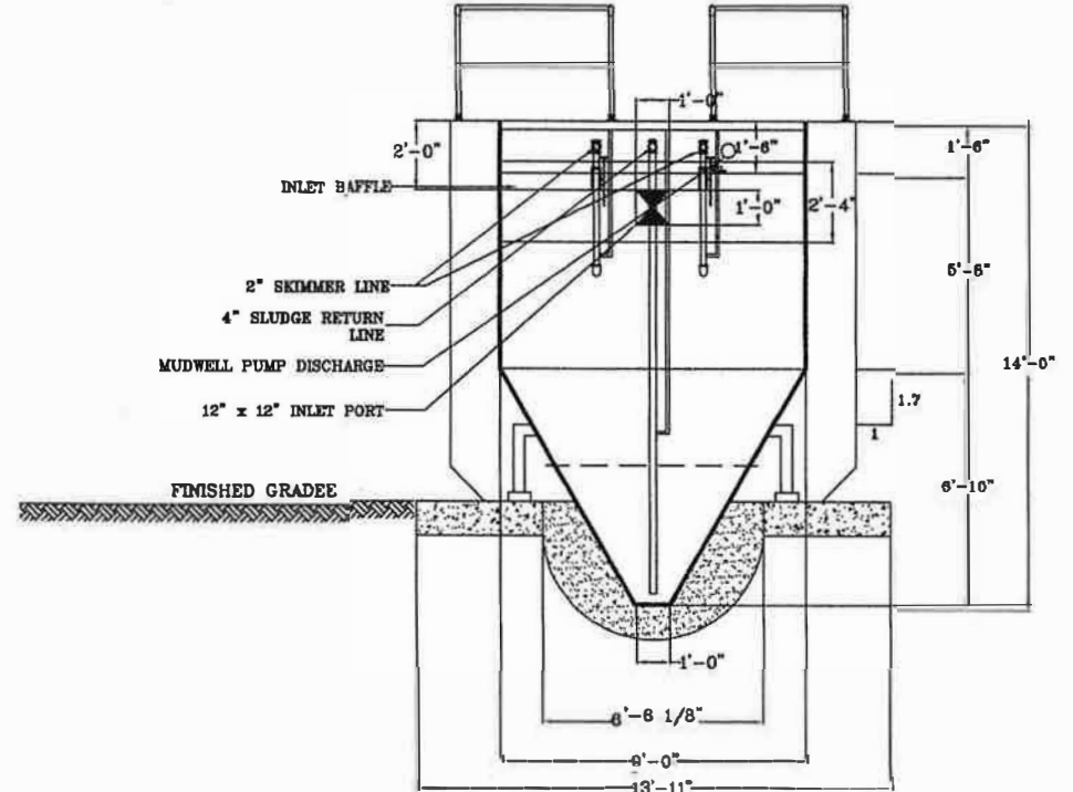
SECTION J-J CLARIFIER INLET END
