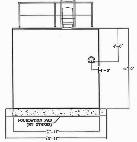
ELEVATION -I-I CL2 TANK
